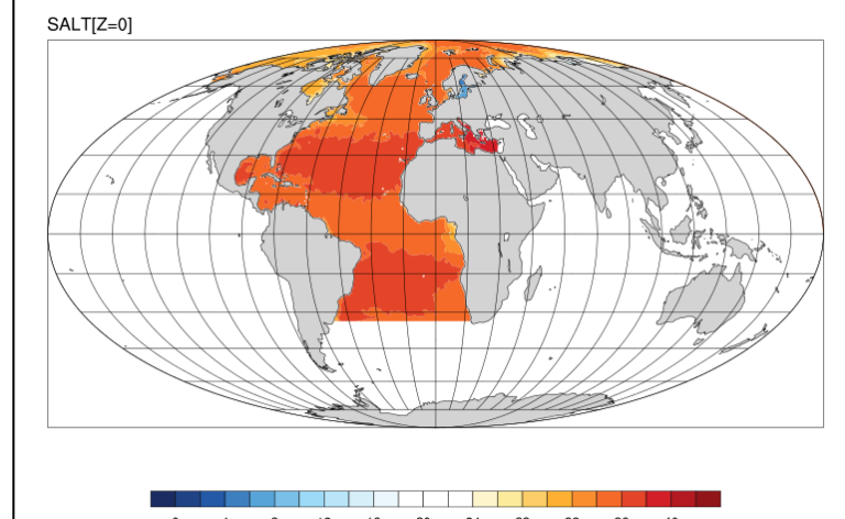
DKRZ NCL Tutorial Example: Mollweide projection
